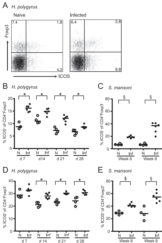
Figure 1. Fcpx3 + Treg cells and Fcpx3 - Tcfx cells increase expression of ICOS in response to helminth infection. C57BL/6 mice were infected with H. polygyrus or S. mansoni and the expression of ICOS by CD4 + Fcpx3 + Treg cells and CD4 + Fcpx3 - Tcfx cells assessed over time. (A) Representative staining for Fcpx3 and ICOS on MLN CD4 + T cells from naïve and H. polygyrus -infected mice 14 day pi. (B, C) Percentage of CD4 + Fcpx3 - cells expressing ICOS from (B) the MLNs of H. polygyrus -infected mice and (C) spleen of S. mansoni -infected mice. (D, E) Percentage of CD4 + Fcpx3 + cells expressing ICOS from (D) the MLNs of H. polygyrus -infected and (E) spleen of S. mansoni -infected mice. Symbols denote individual naïve (open) and infected (closed) mice, and lines denote means (B, D) or medians (C, E). Results show one representative experiment of two performed for each time point. * p < 0.005 (ANOVA using combined data from two separate experiments). § p < 0.05 (Mann–Whitney).
