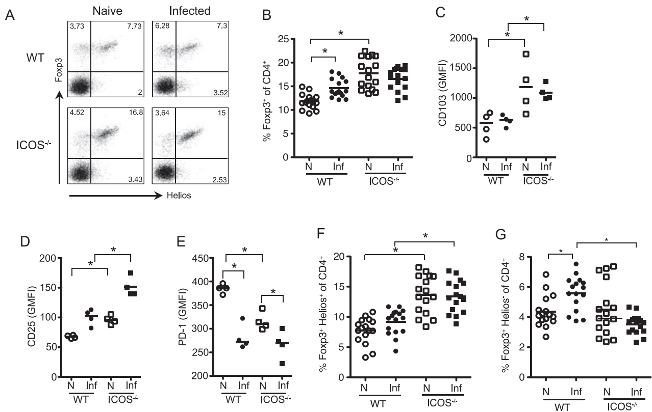
Figure 3. ICOS -/- mice show impaired expansion of Helios - Foxp3 + Treg cells within the LP. WT (circles) and ICOS -/- (squares) mice were infected with H. polygyrus and the expression of Fxp3, CD103, CD25, PD-1 and Helios by LP CD4 + T cells assessed at day 7 pi. (A) Representative staining for Fxp3 and Helios on CD4 + T cells. (B) Percentage of LP CD4 + T cells expressing Fxp3 was determined by flow cytometry. (C–E) Geometric mean expression intensity of (C) CD103, (D) CD25 and (E) PD-1 on CD4 + Fxp3 + Treg cells. (F and G) Percentage of (F) Helios + Fxp3 + and (G) Helios - Fxp3 + Treg cells is shown. Data shown are from (B, F, G) four independent experiments or from (C, D, E) one experiment representative of three performed. Open symbols represent naive mice and closed symbols represent infected WT mice. * p < 0.05 (Tukey HSD, ANOVA performed using combined data from three or four experiments).
